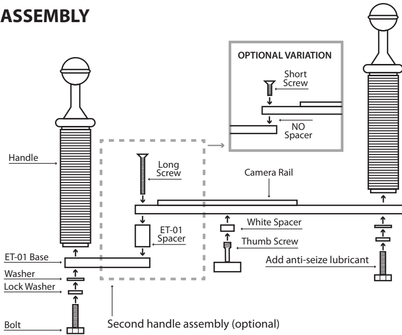
HB-01 or HB-05 Handle
